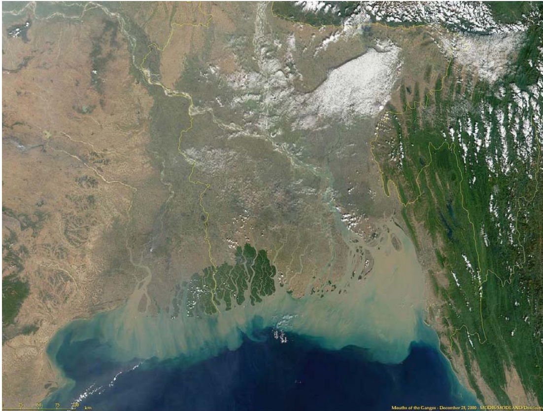
Figure 3. The mouths of the Ganges-Brahmaputra-Megna Rivers. (Courtesy of NASA at http://oceancolor.gsfc.nasa.gov ).
